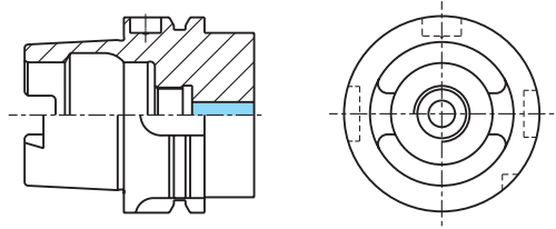
ISO12164 - 3 - HSK - T
